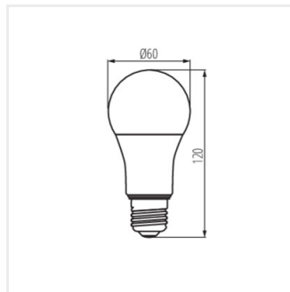
IQ-LED A60 11W-WW
